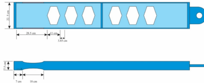
Figure 1. Castellated beam designs of previous research.
